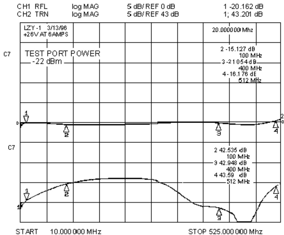
Figure 1: Small Signal Response @ -22 dBm P IN
