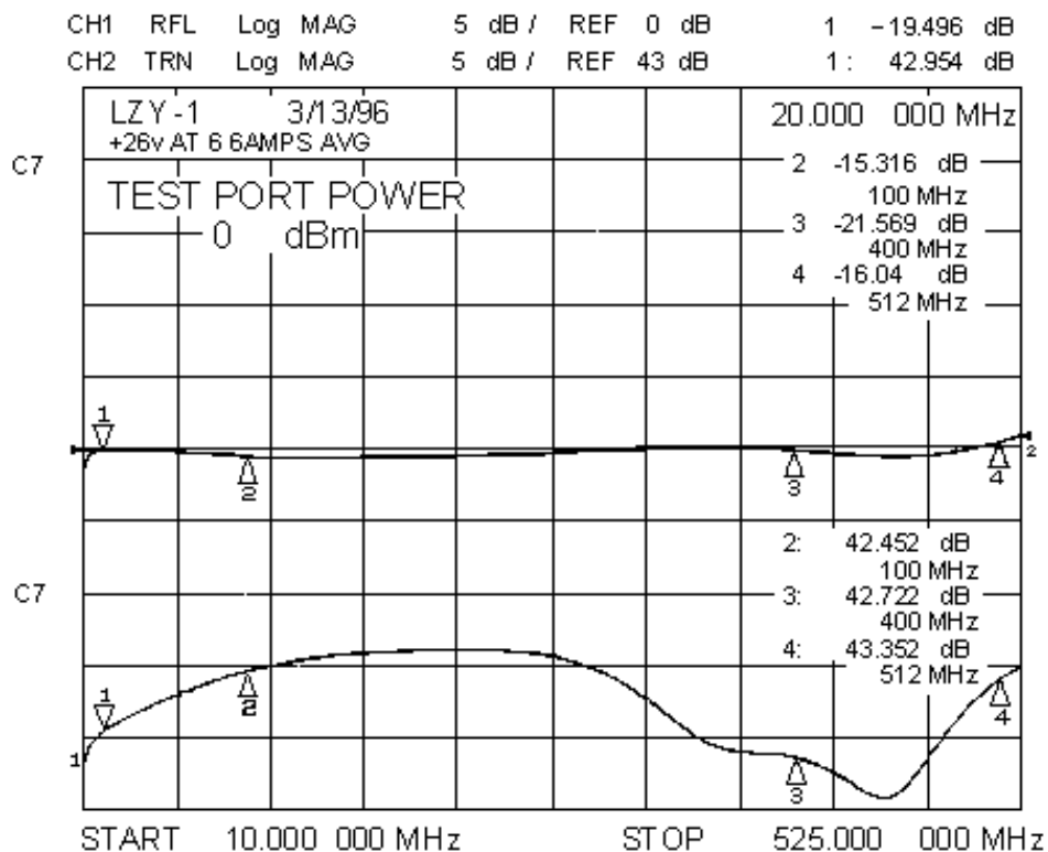
Figure 2: Large Signal Response @ 0 dBm P IN
