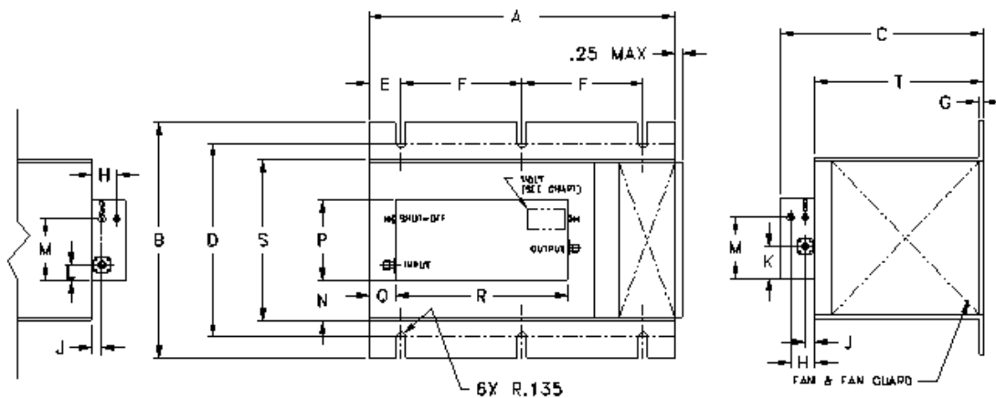
Mechanical Outline Drawing & Dimensions
