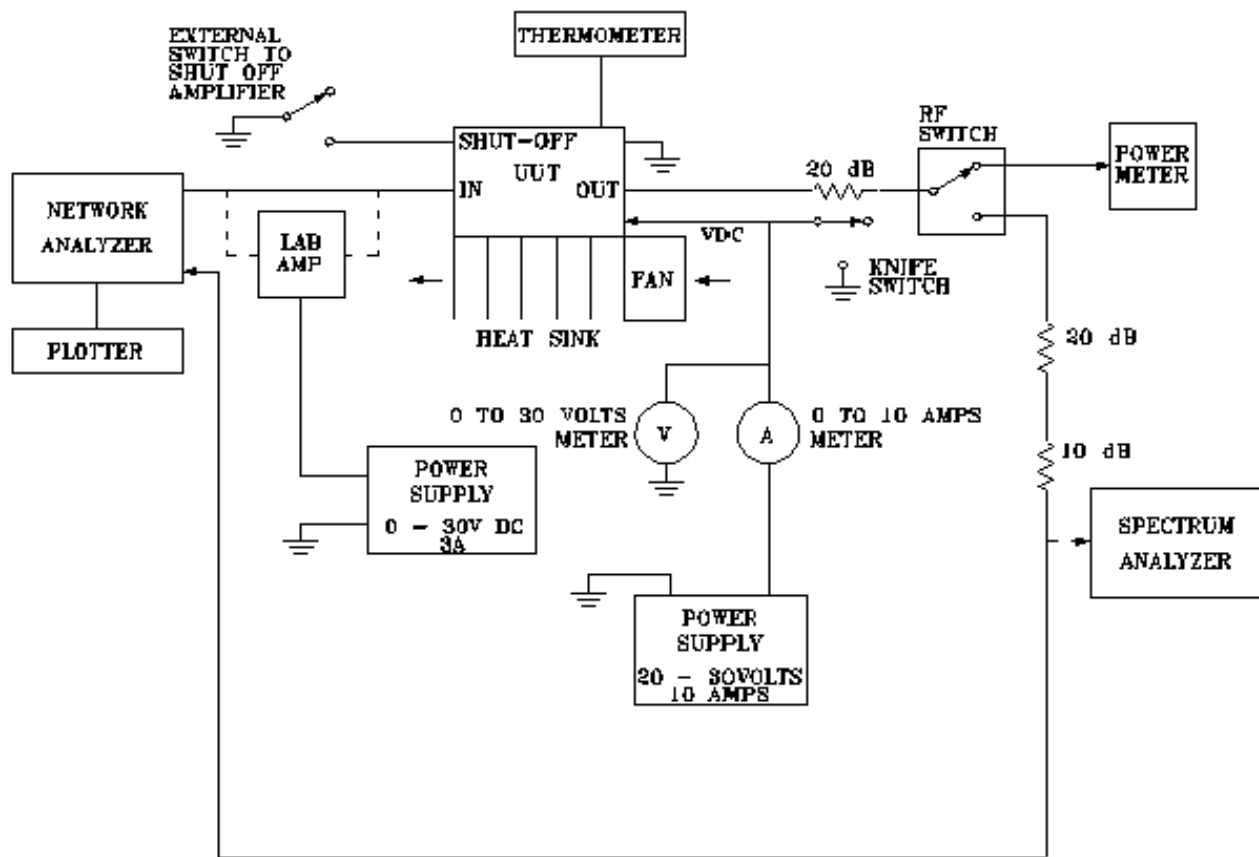
Figure 3: Acceptance Test Procedure Test Setup
